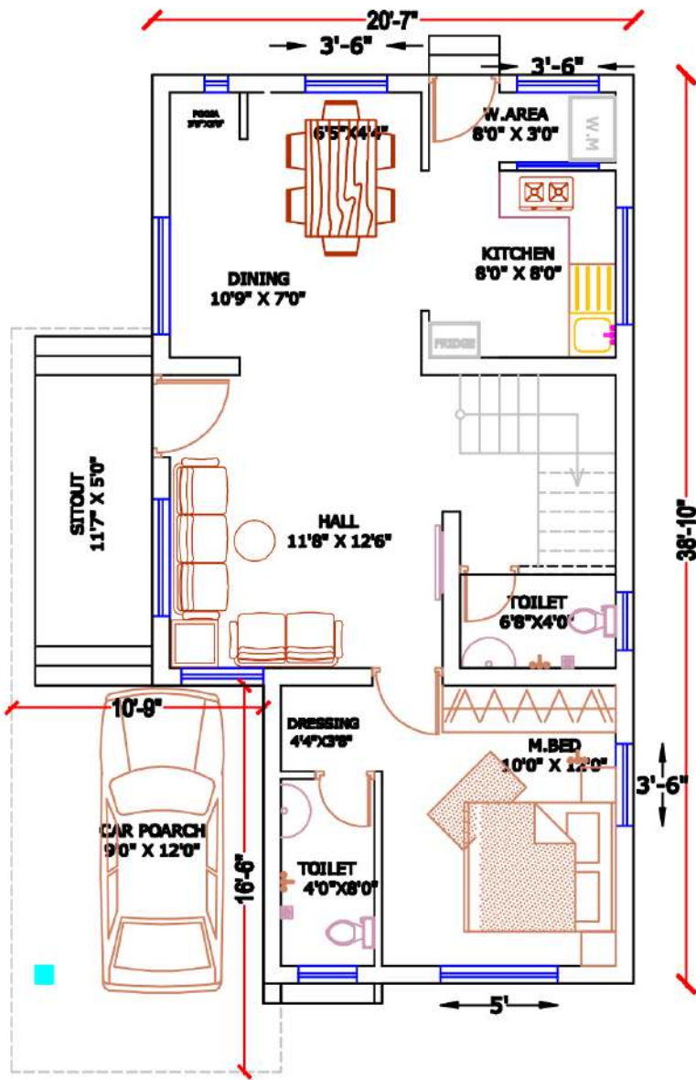
GROUND FLOOR
