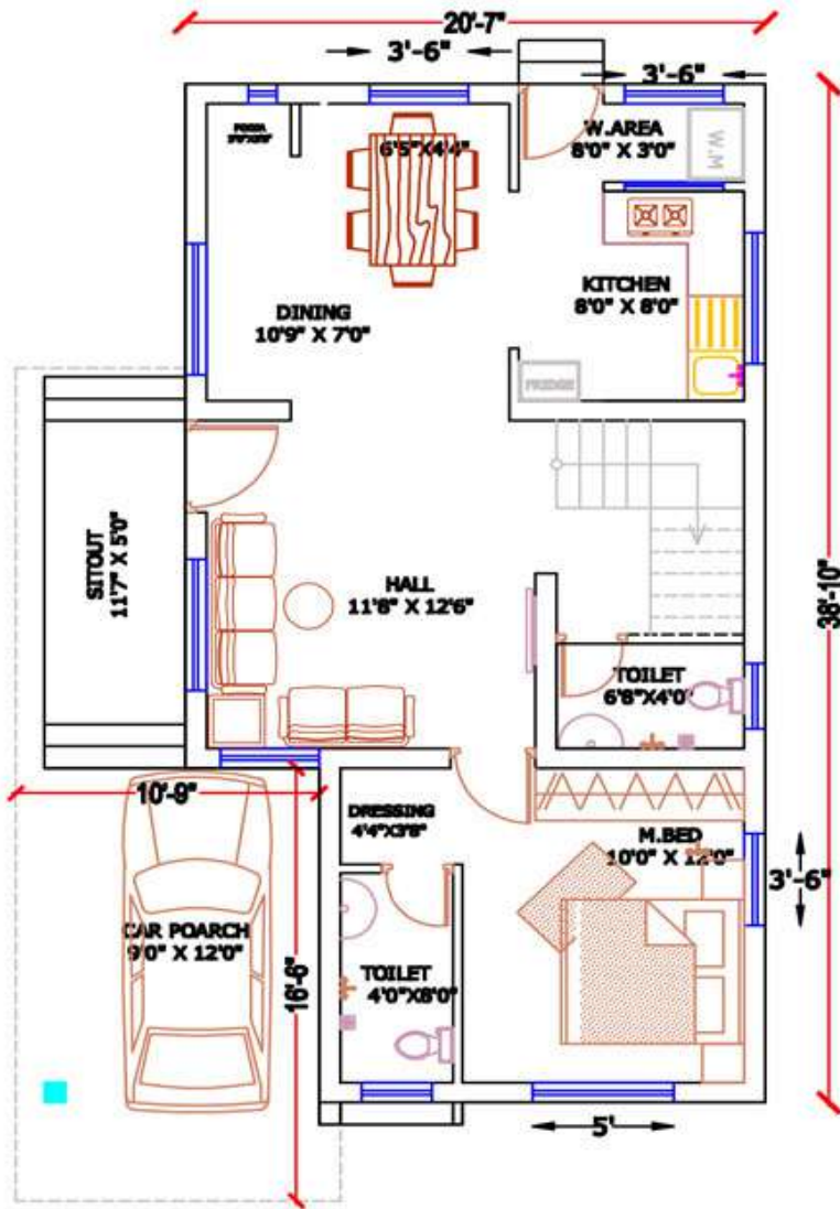
GROUND FLOOR
